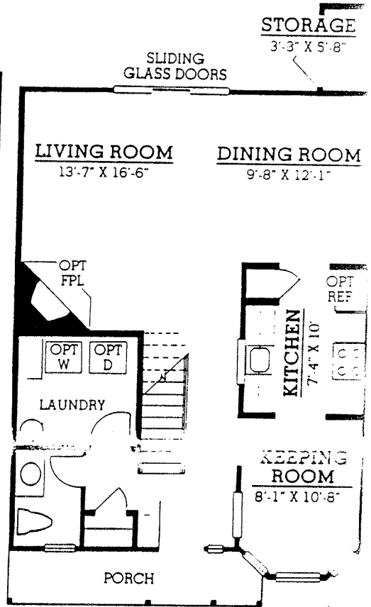
ALTERNATE FIRST FLOOR INTERIOR
